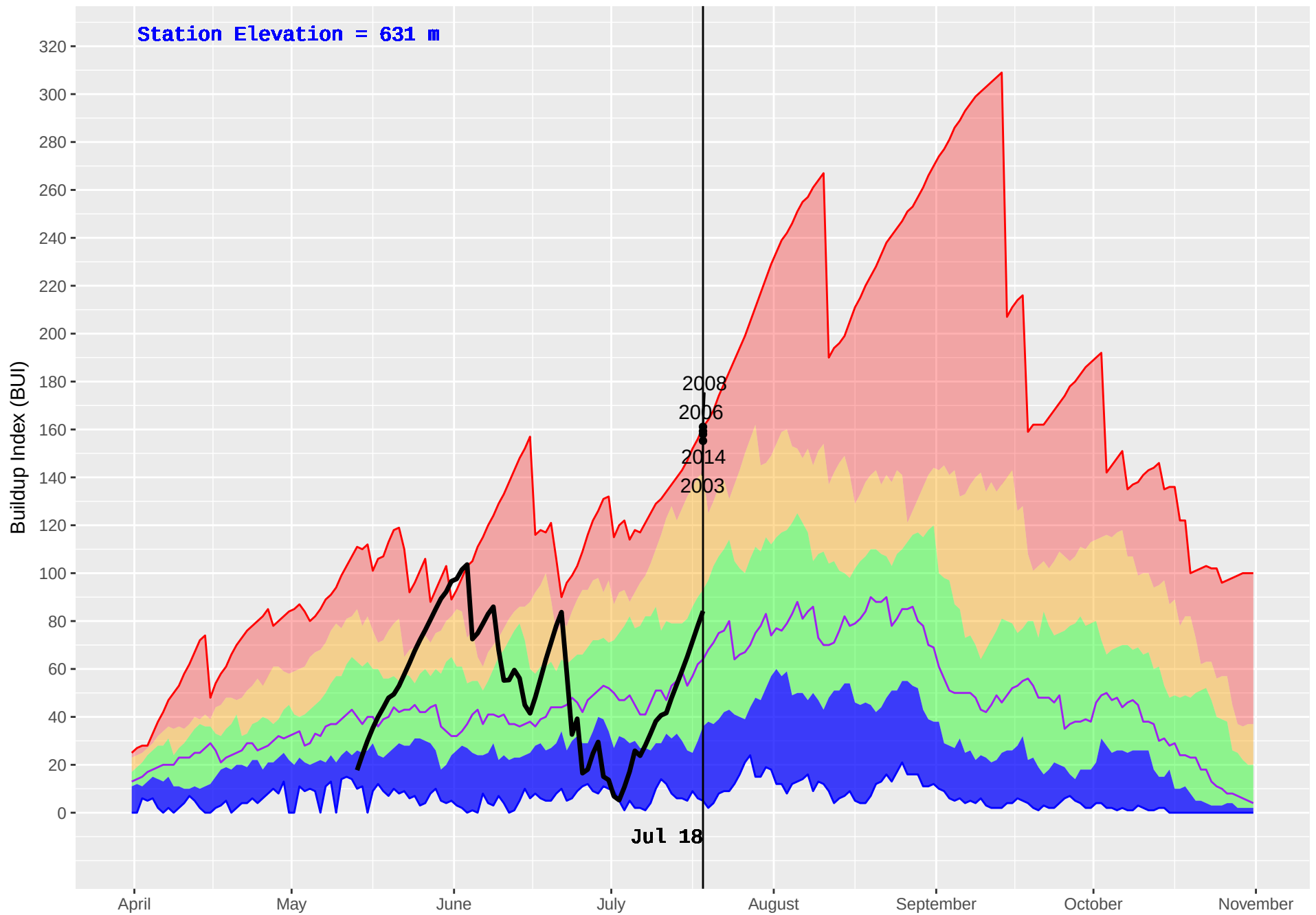
EAST BARRIERE (243) : Historical (1978–2016) and Current (2018) Daily Buildup Index (BUI)
