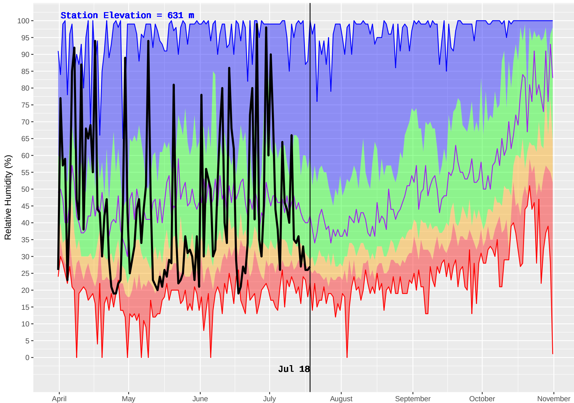
EAST BARRIERE (243) : Historical (1978–2016) and Current (2018) Daily Relative Humidity
